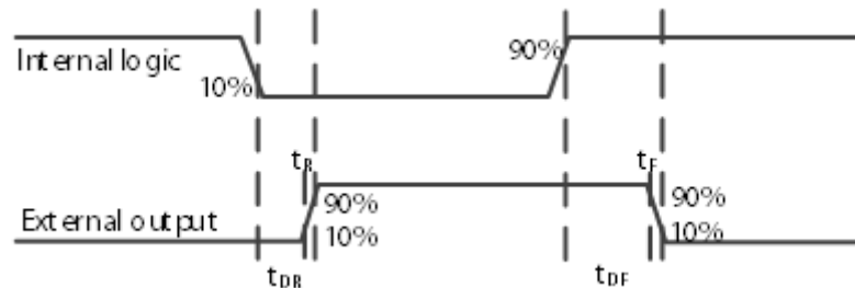
Figure 3-23 Delay time of rising and falling
