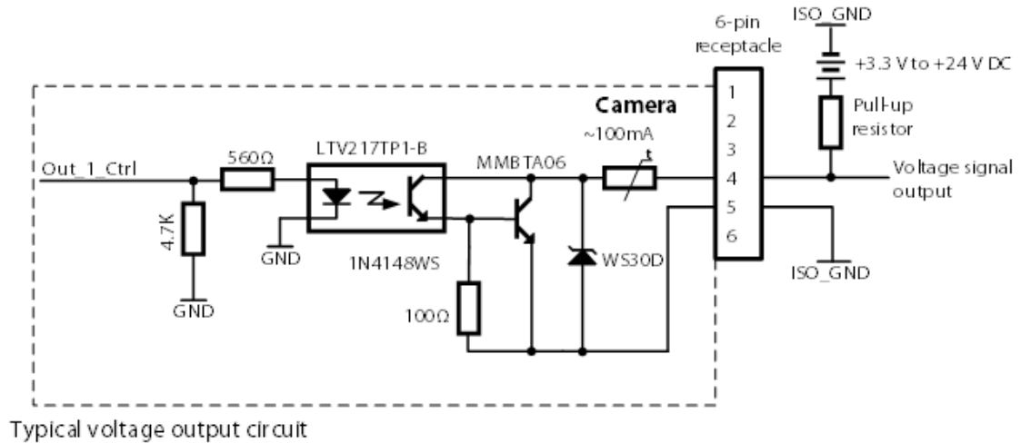
Figure 3-22 Internal circuit of Line0
