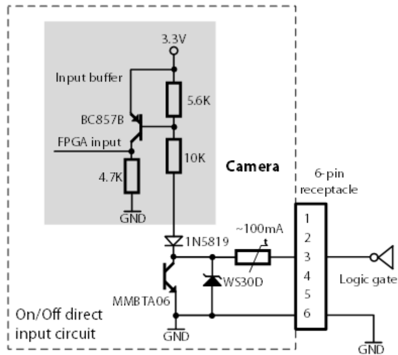
Figure 3-19 5 VTTL logic level input circuit
